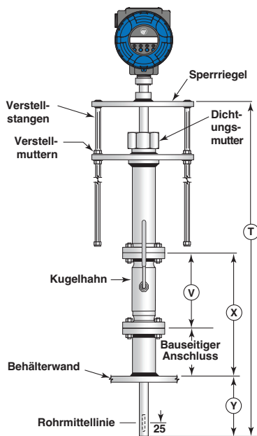
Modell RPA-F412-XXX
